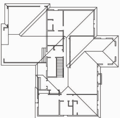
ROOF PLAN SCALE: 1/8" = 1'-0"
